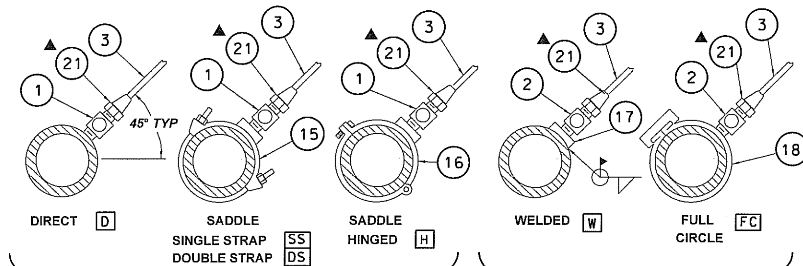
CORPORATION STOP THREADS (CC)
