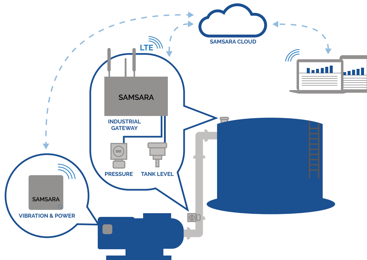
Figure 8. Pump Efficiency System
